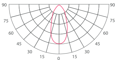
LIGHTING DISTRIBUTION CURVE
